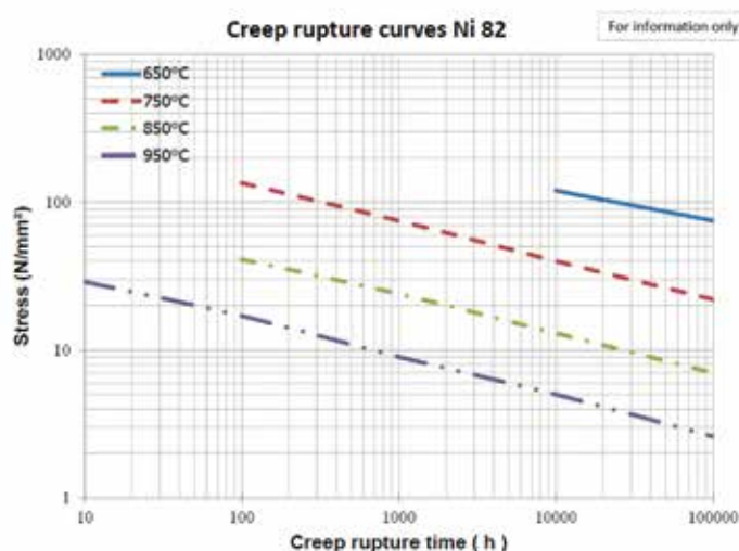
Example of Creep Resistance graphic
